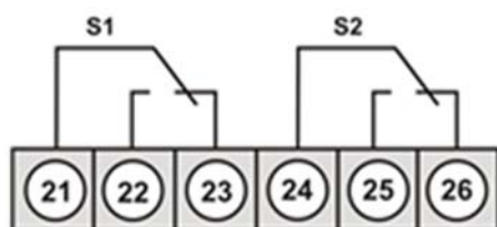
Relay Option
