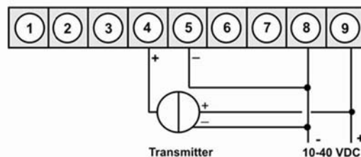
DAG-M4V in combination with a 3-wire sensor 0/4-20 mA
