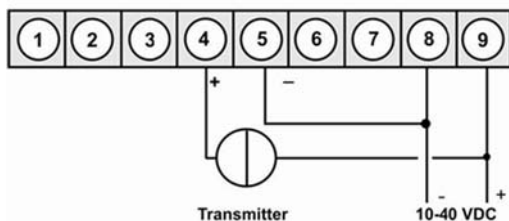
DAG-M4V in combination with a 3-wire sensor 0-10 V
