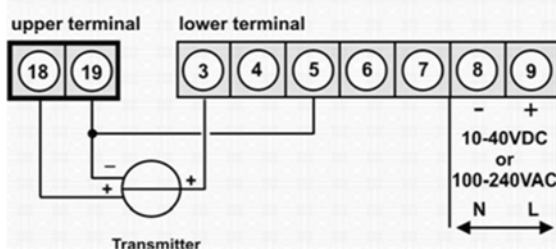
3-wire sensor 0-10 V
