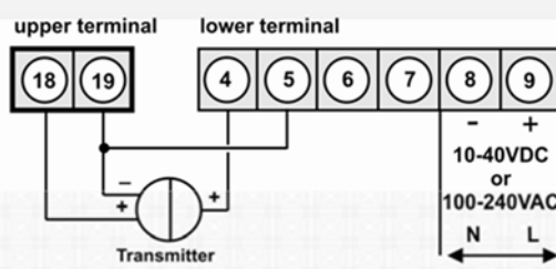
3-wire sensor 0-20 mA
