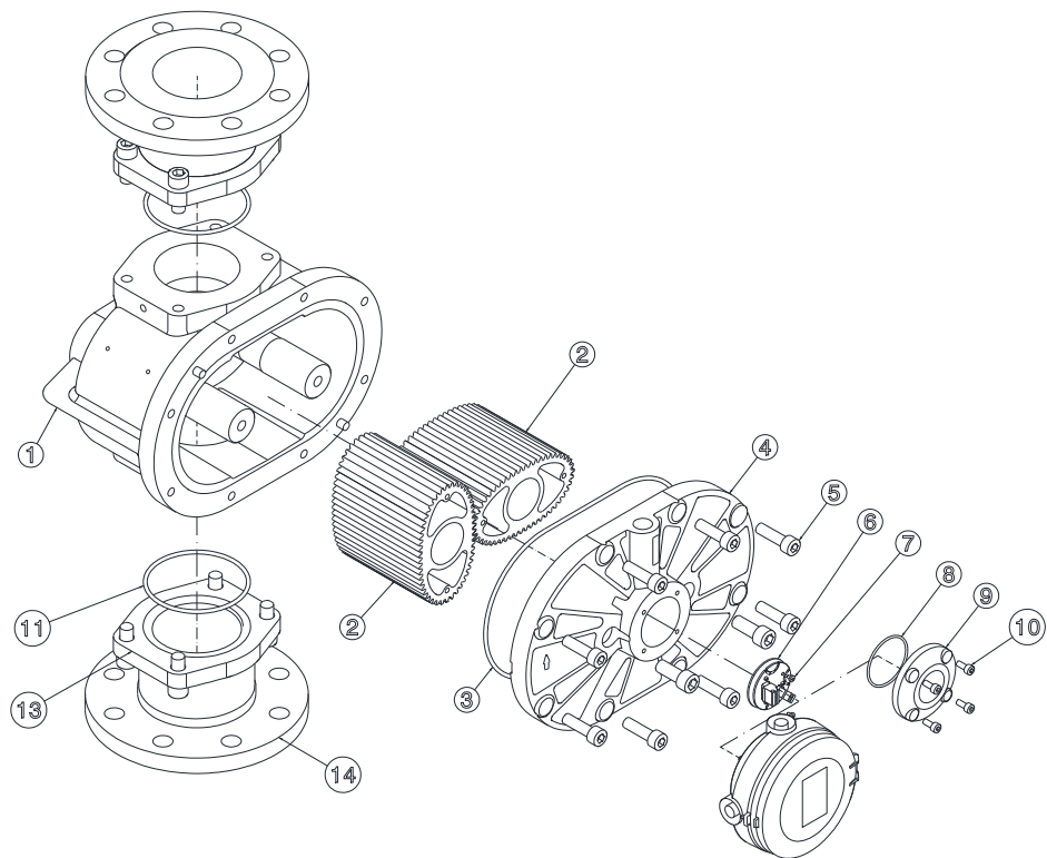
Exploded view of DON-x45...DON-x60
